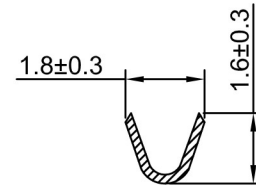
B-B SECTION
